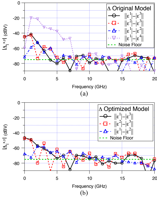
Fig. 6: Magnitude of \Delta_1^{x,y} for the parallel diode case for (a) the original SPICE model and (b) a model optimized to measurements. Subscripts in the figure legend are omitted for clarity.
