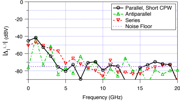
Fig. 5: Magnitude of \Delta_1^{1,3} = |\varepsilon_1^1| - |\varepsilon_1^3| for the three diode configurations described in Table 1.
